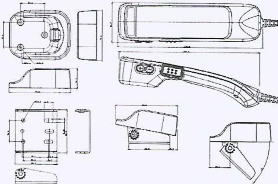
Handset Mechanical Dimension
