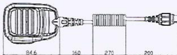
Fist MIC Cable and Connector
