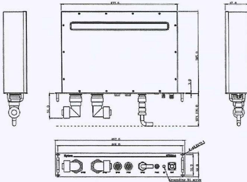
TRIU Cabling
