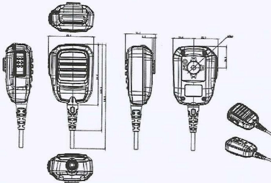
Fist MIC Mechanical Dimension
