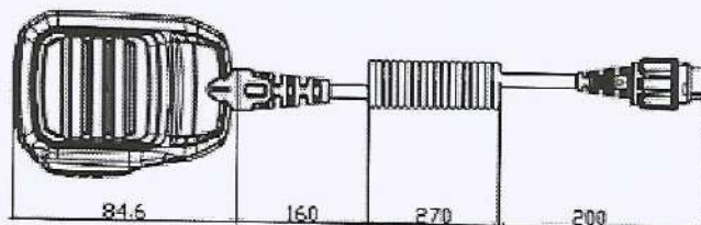
Fist MIC Cable and Connector
