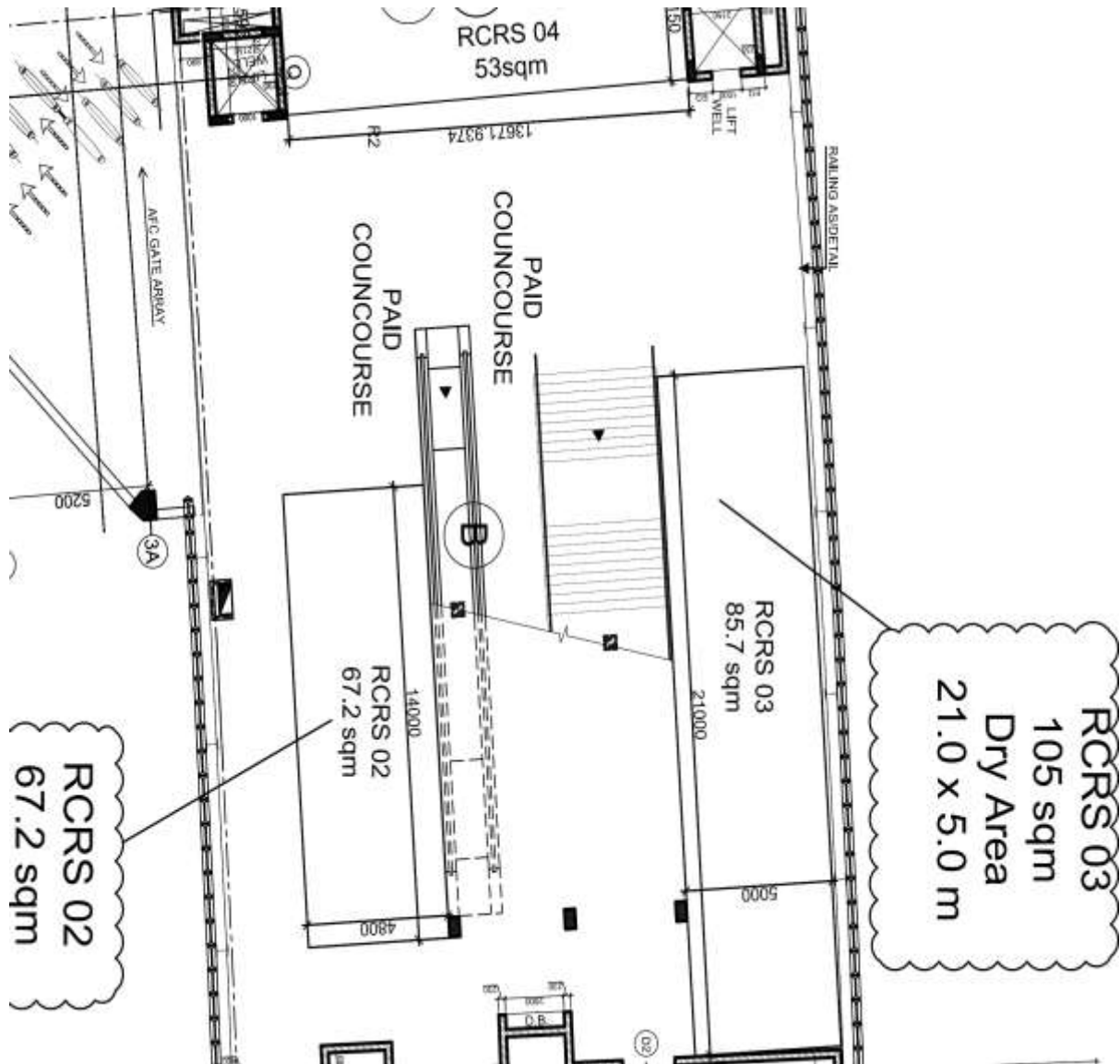
RCRS-03 (Area = 105.00 Sqm.)
